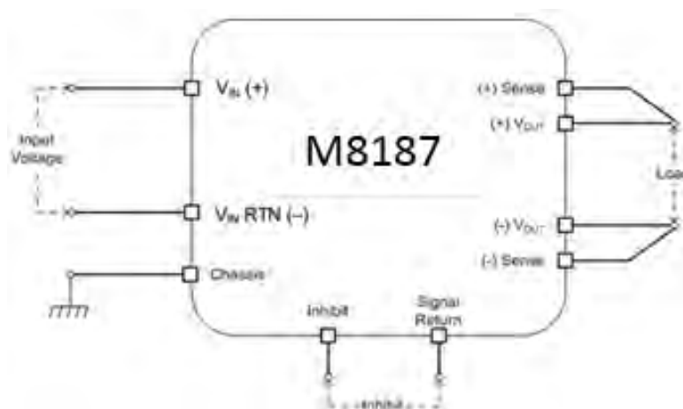
FIGURE 1: CONNECTION DIAGRAM:
