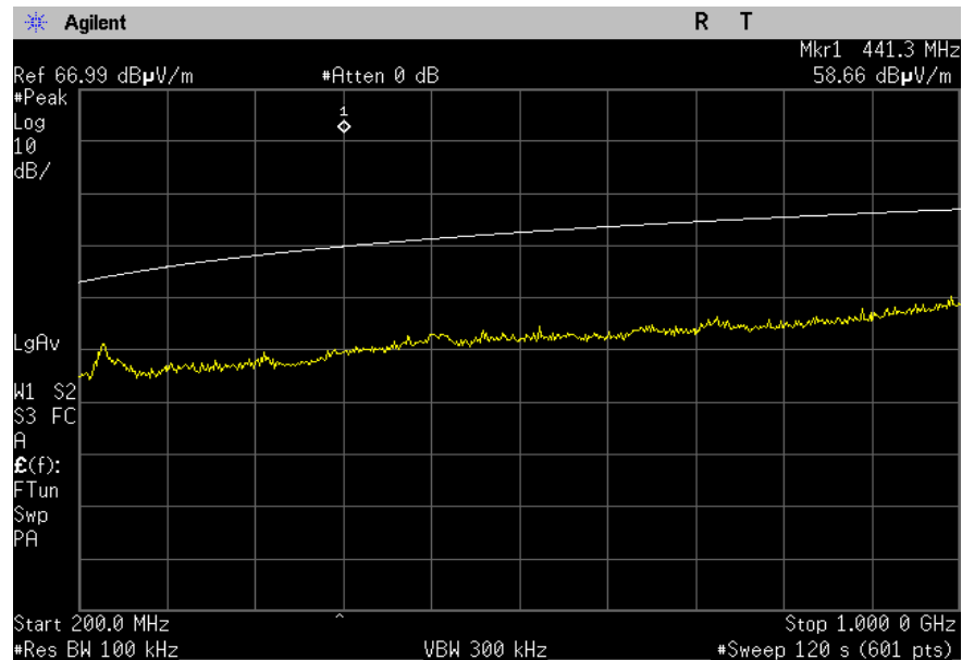
Plot 1.8: RE102 test results within 200 – 1000 MHz, vertical polarization
