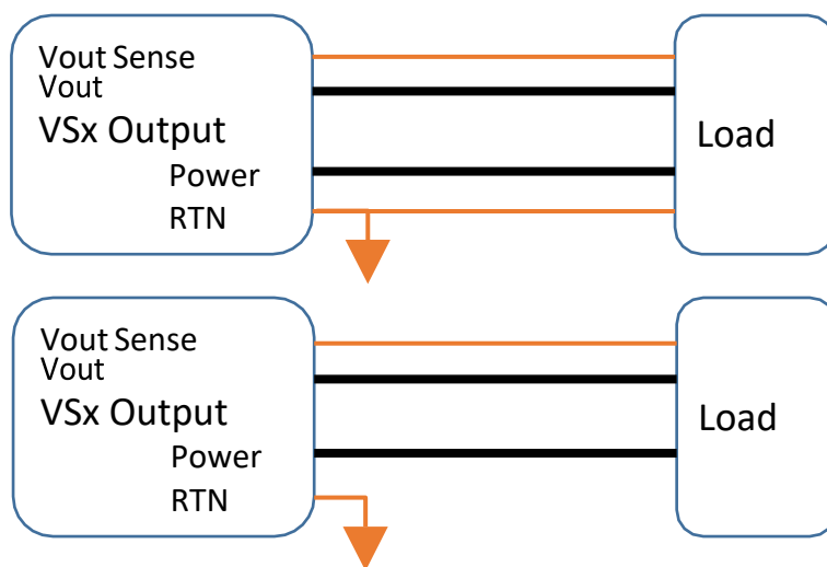
Figure 2: Sense line connection
