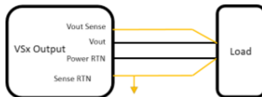
Figure 3: M4705 Sense line connection
